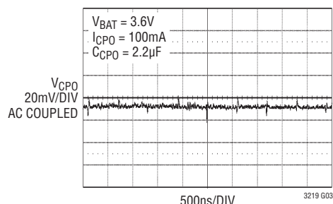
2x Mode CPO Ripple
