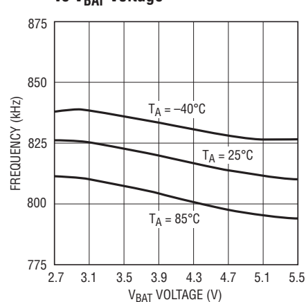
Oscillator Frequency vs V_{\text{BAT}} Voltage
