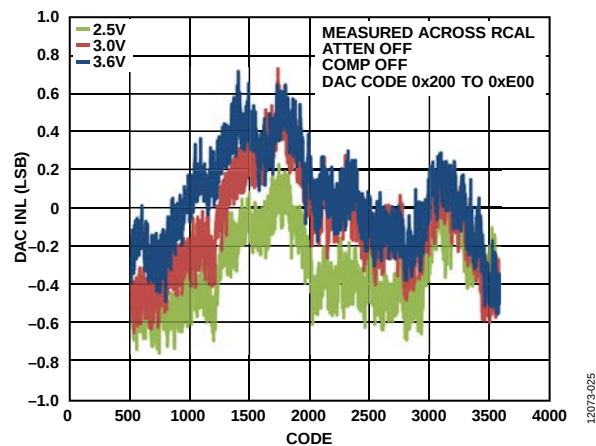
Figure 25. DAC INL (12-Bit) vs. Code
