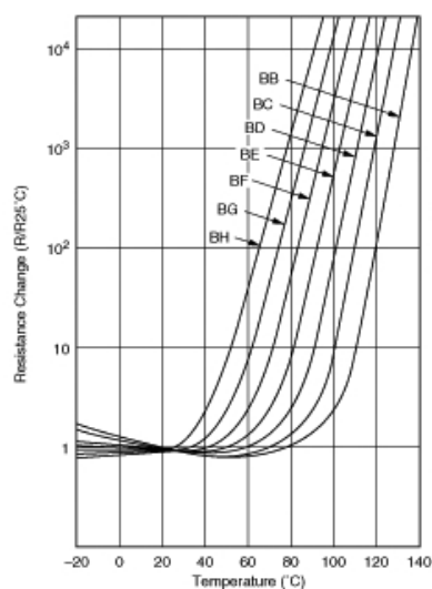
Resistance-Temperature Characteristics
