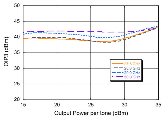
Output IP3 vs. Output Power per Tone
