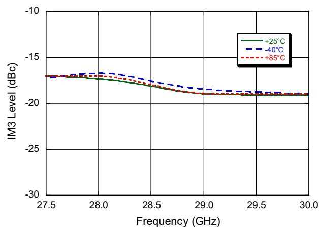
IM3 vs. Frequency over Temperature ( P_{OUT} = +33 dBm/Tone)
