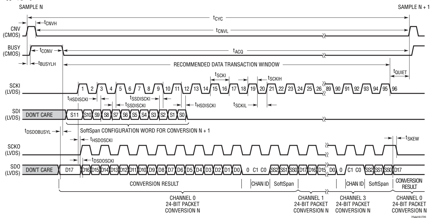
Figure 20. Serial LVDS I/O Mode
