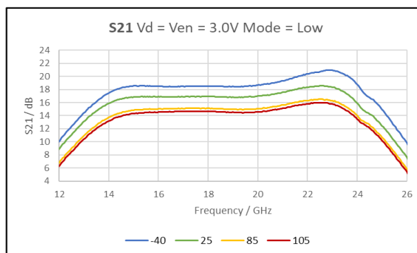
Figure 30: S21 V_d = V_{en} = 3V , low current mode
