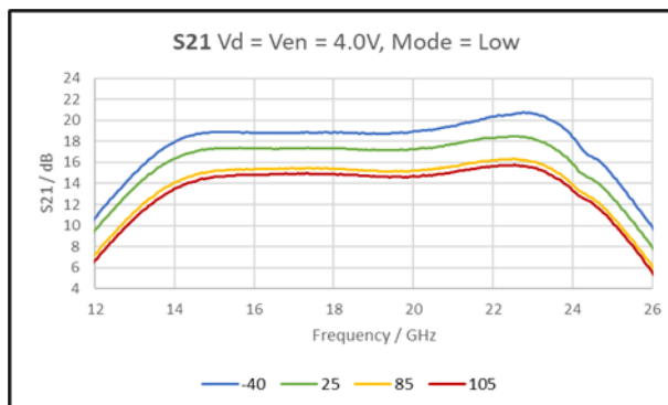
Figure 28: S21 V_d = V_{en} = 4.0V , low current mode
