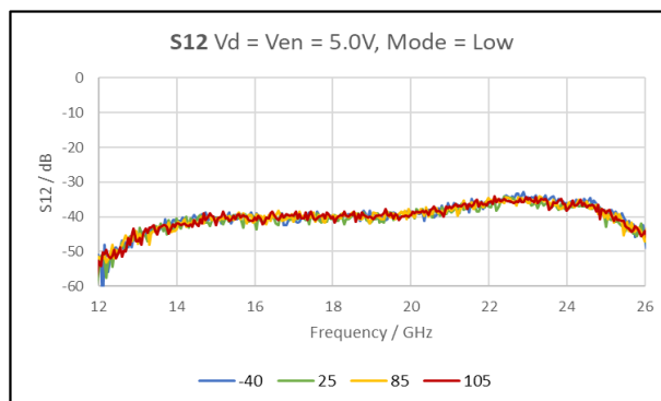
Figure 32: S12 V_d = V_{en} = 5.0V , low current mode
