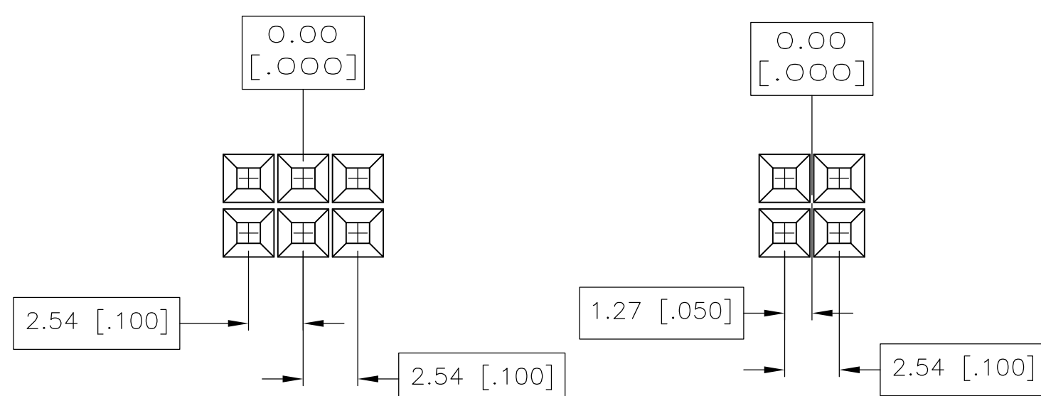
DETAIL Z
