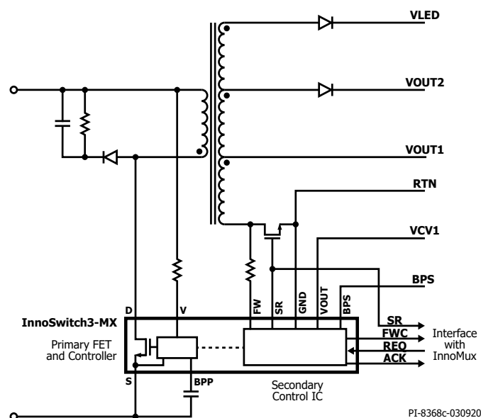
Figure 1. Typical Application/Performance.
