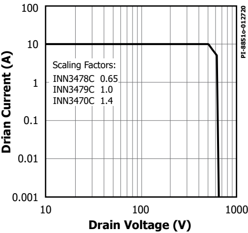
Figure 11. Maximum Allowable Drain Current vs. Drain Voltage (PowiGaN Devices INN3478C / INN3479C / INN3470C).
