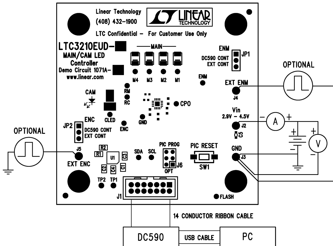
Figure 1. Proper Measurement Equipment Setup for DC1071A
