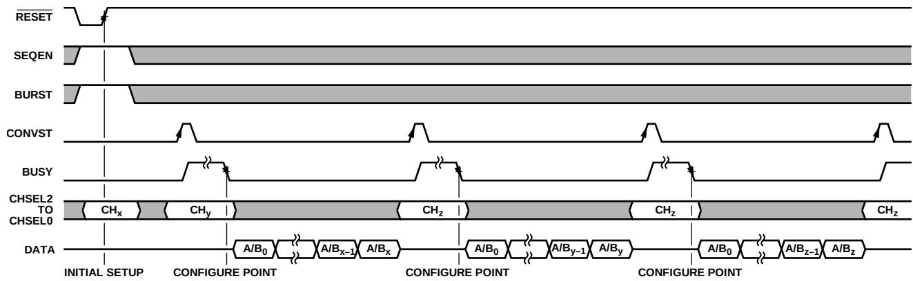
Figure 56. Burst Sequencer, Hardware Mode
