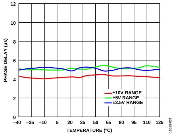
Figure 31. Phase Delay vs. Temperature
