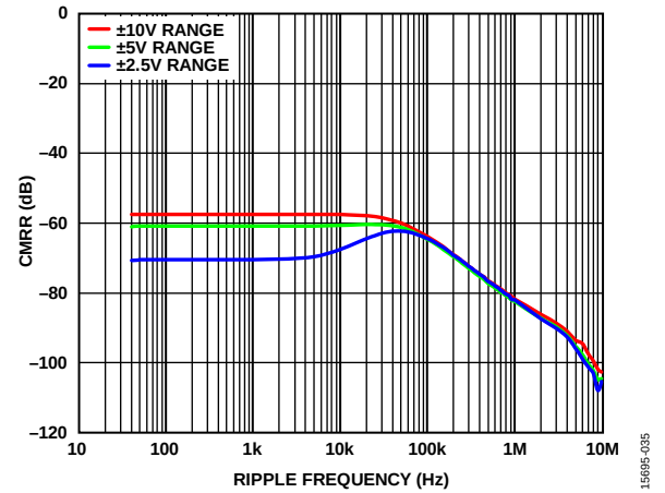
Figure 35. CMRR vs. Ripple Frequency
