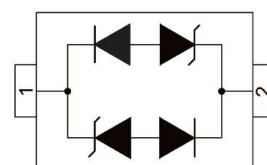
PIN Configuration
