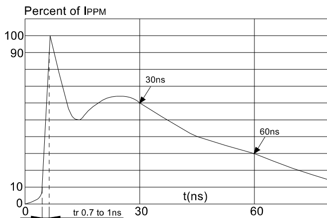
FIG.4: ESD clamping
