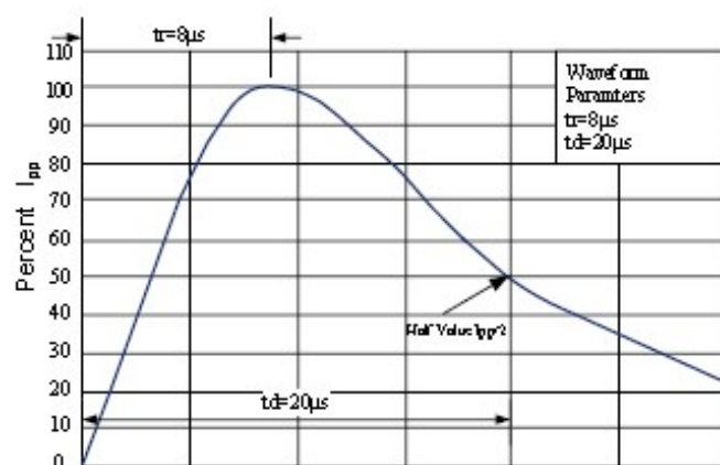
Figure 5: Pulse Waveform
