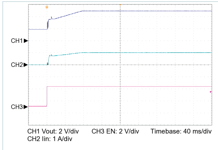
Figure 15 — Startup from EN, V_{IN} = 270\text{ V} , C_{OUT\_EXT} = 10000\text{ }\mu\text{F} , R_{LOAD} = 0.100\text{ }\Omega
