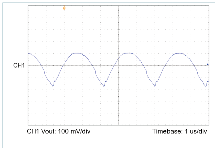
Figure 17 — Output voltage ripple, V_{IN} = 270\text{ V} , V_{OUT} = 5.0\text{ V} , C_{OUT\_EXT} = 1000\text{ }\mu\text{F} , R_{LOAD} = 0.100\text{ }\Omega
