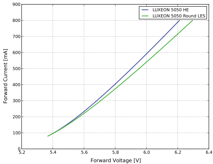
Figure 4a. Typical forward current vs. forward voltage for L150-xxxx500600000 and L150-xxxx500600xH0, T j =25°C.
