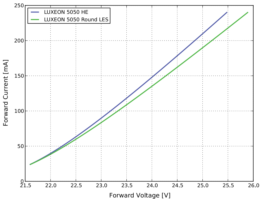
Figure 4b. Typical forward current vs. forward voltage for L150-xxxx502400000 and L150-xxxx502400xH0, T j =25°C.
