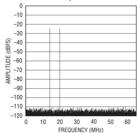
32k Point 2-Tone FFT, f_{IN} = 20.14\text{MHz} and 14.25MHz, -25dBFS, PGA = 0, RAND = "On", Dither "Off"
