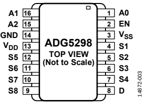
Figure 3. Reversed Formed FLATPACK Pin Configuration
