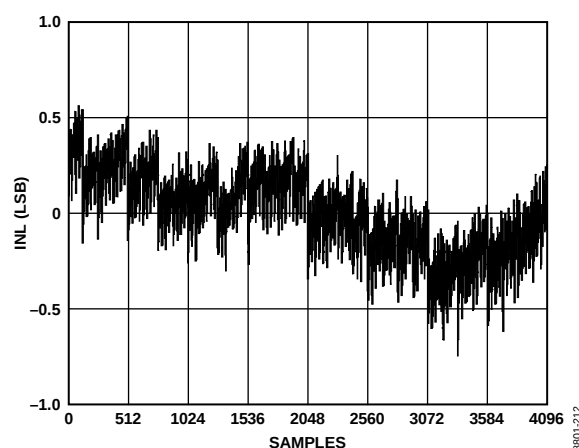
Figure 15. Auxiliary ADC INL
