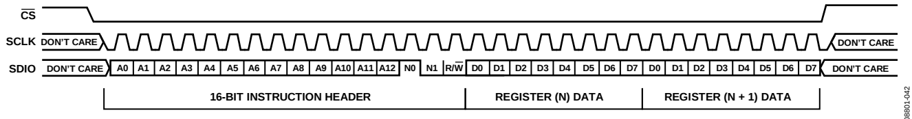
Figure 37. Serial Control Port Access—LSB First, 16-Bit Instruction, Two Bytes Data
