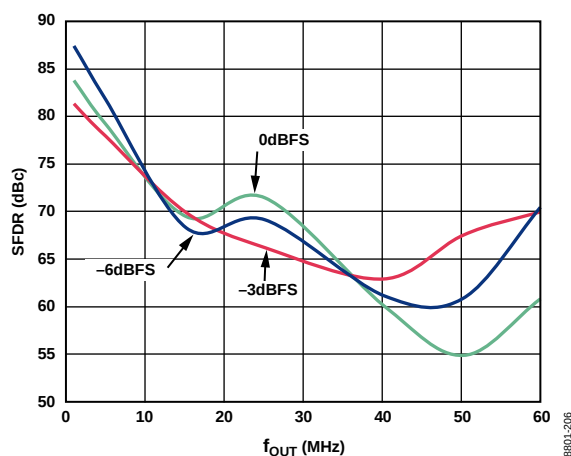
Figure 9. Third Harmonic Distortion vs. f_{OUT} Over Digital Scale, f_{DAC} = 125 MHz, 1 \times , Full-Scale Current = 2 mA, TXVDD = 1.8 V
