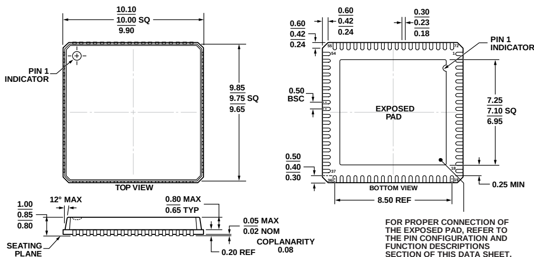
COMPLIANT TO JEDEC STANDARDS MO-220-VNND-4 Figure 104. 72-Lead Lead Frame Chip Scale Package [LFCSP_VQ] 10 mm x 10 mm Body, Very Thin Quad (CP-72-4) Dimensions shown in millimeters
