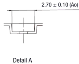
Figure 9. SKY66114-11 Tape and Reel Dimensions
