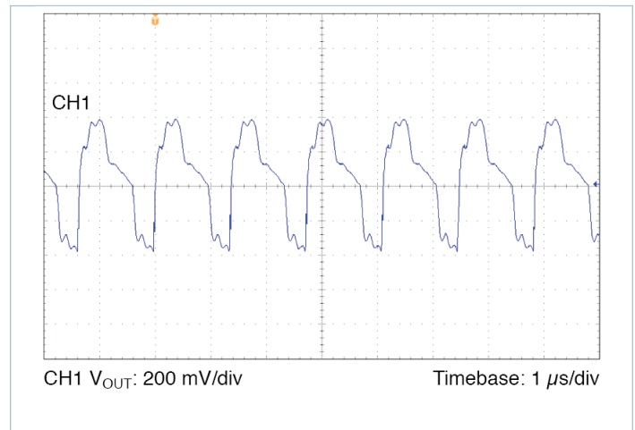
Figure 19 — Output voltage ripple, V_{IN} = 48\text{ V} , V_{OUT} = 36.0\text{ V} , C_{OUT\_EXT} = 220\text{ }\mu\text{F} , R_{LOAD} = 4.045\text{ }\Omega
