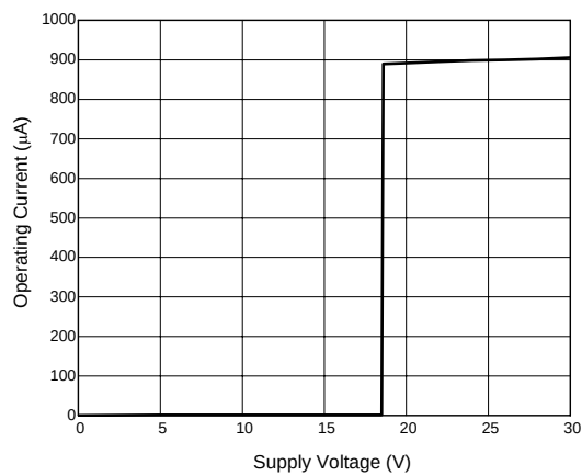
Figure 8. Operating Current vs. Supply Voltage
