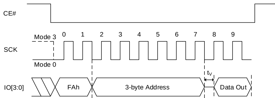
Figure 8.76 Read DQB Sequence In QPI Mode (FAh)
