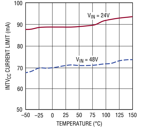
INTV CC Current Limit vs Temperature
