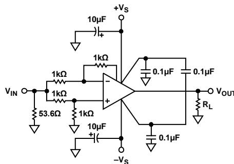
Figure 51. Common-Mode Rejection
