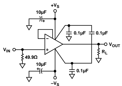
Figure 46. G = 1 Configuration
