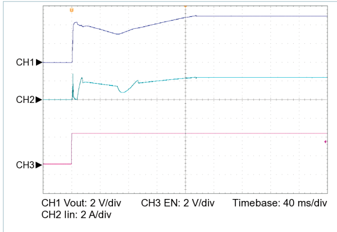
Figure 15 — Startup from EN, V_{IN} = 48\text{ V} , C_{OUT\_EXT} = 10000\text{ }\mu\text{F} , R_{LOAD} = 0.156\text{ }\Omega
