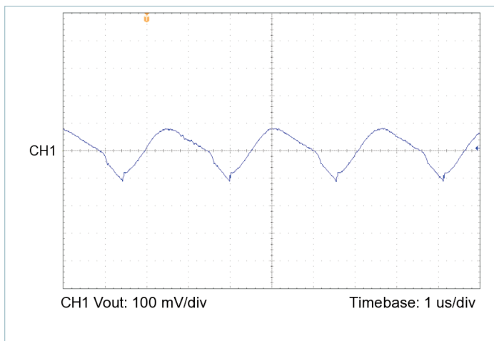
Figure 17 — Output voltage ripple, V_{IN} = 48\text{ V} , V_{OUT} = 5.0\text{ V} , C_{OUT\_EXT} = 1000\text{ }\mu\text{F} , R_{LOAD} = 0.156\text{ }\Omega
