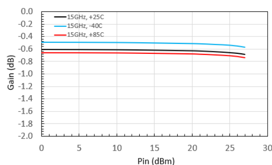
Input Power Compression (Insertion Loss @ 15 GHz)
