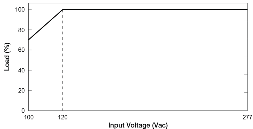
Fig. 2 De-rating for Low Input Voltage (All Models) < 120Vac de-rate power by 1.5% / Vac
