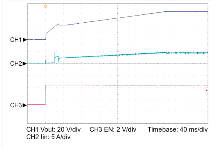
Figure 15 — Startup from EN, V_{IN} = 48\text{ V} , C_{OUT\_EXT} = 2200\text{ }\mu\text{F} , R_{LOAD} = 7.200\text{ }\Omega
