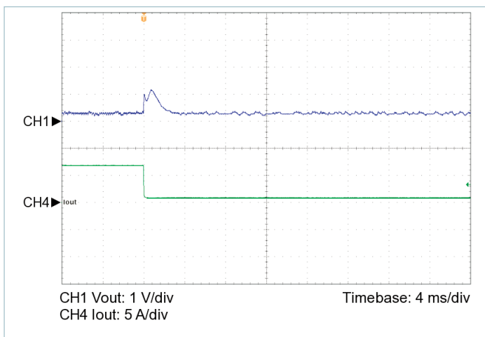
Figure 5 — 100% to 10% load transient response, V_{IN} = 48\text{ V} , nominal trim, C_{OUT\_EXT} = 220\text{ }\mu\text{F}
