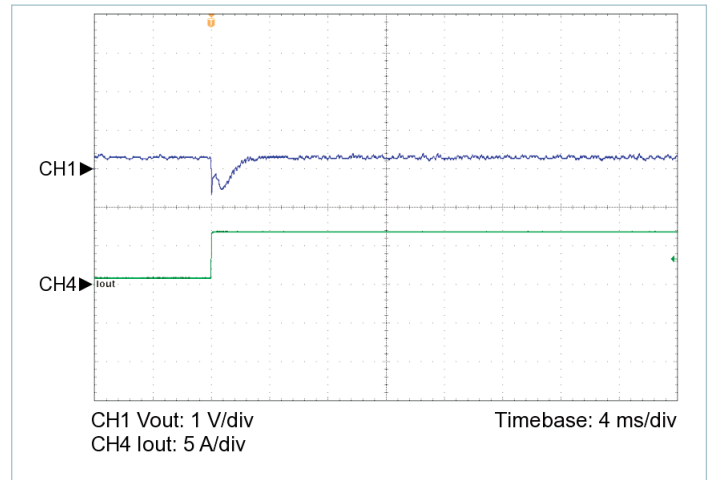
Figure 6 — 10% to 100% load transient response, V_{IN} = 48\text{ V} , nominal trim, C_{OUT\_EXT} = 220\text{ }\mu\text{F}
