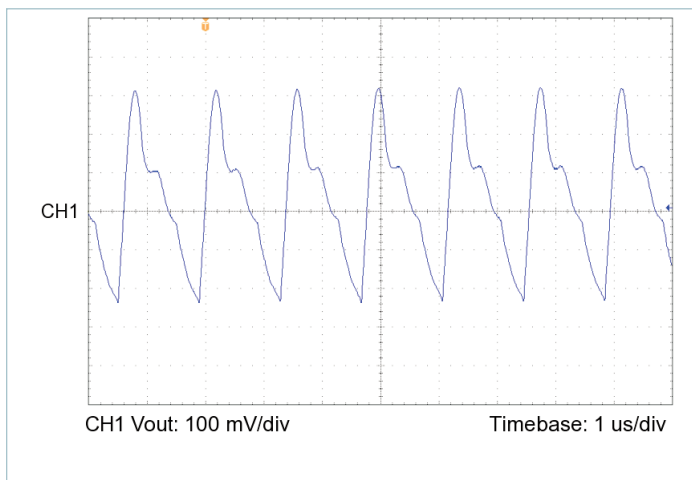
Figure 17 — Output voltage ripple, V_{IN} = 48\text{ V} , V_{OUT} = 48.0\text{ V} , C_{OUT\_EXT} = 220\text{ }\mu\text{F} , R_{LOAD} = 7.200\text{ }\Omega
