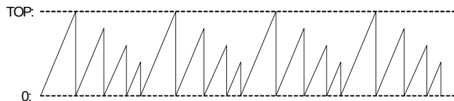
Figure 34-6. Counter in Spread-Spectrum Operation
