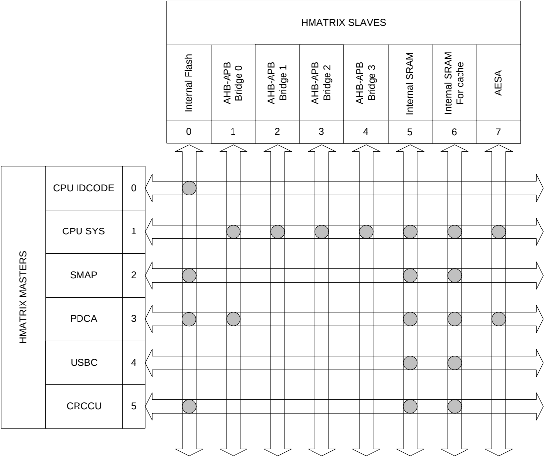
Figure 15-1. HMatrix Master / Slave Connections
