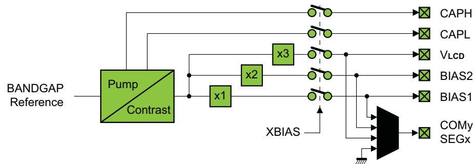
Figure 39-13. LCD Power Supply Block Diagram
