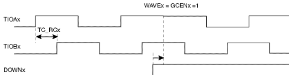
Figure 30-13. 2-bit Gray Up/Down Counter.
