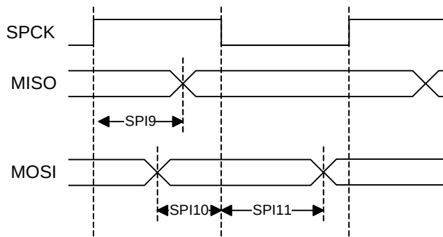
Figure 42-15. SPI Slave Mode with (CPOL= NCPHA= 0) or (CPOL= NCPHA= 1)
