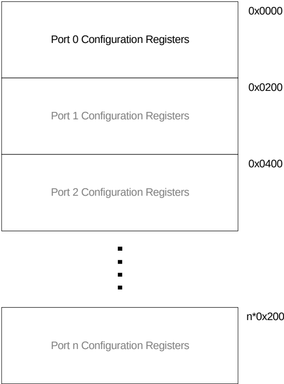
Figure 23-6. Port Configuration Registers
