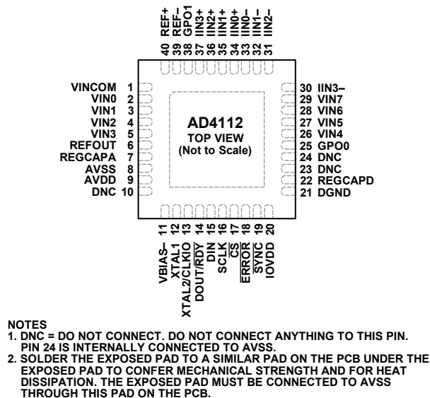
Figure 4. Pin Configuration
