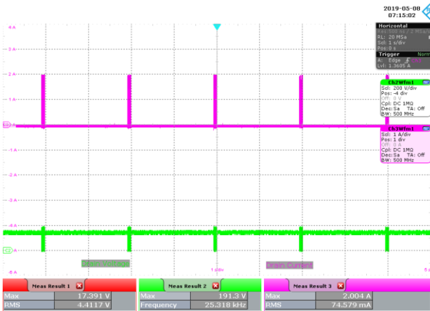
Figure 95 – 100 VAC, Output Shorted. Upper: I_{DRAIN} , 1 A / div. Lower: V_{DRAIN} , 200 V / div., 1 s / div.
