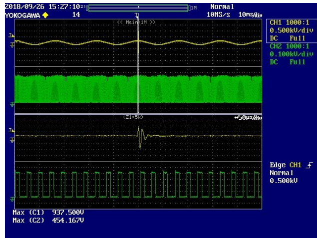
Figure 142 – (+) 2.5 kV Ring Wave Surge, 270° Phase Angle. Lower: V_{DRAIN} , 100 V / div., 10 ms / div. Peak V_{DRAIN} : 454.17 V.
