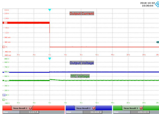
Figure 101 – 100 VAC, 48 V LED Load, Running Open Load. I_{OUT} , 400 mA / div. V_{OUT} , 10 V / div., 4 s / div. PFC V_{OUT} , 100 V / div.
