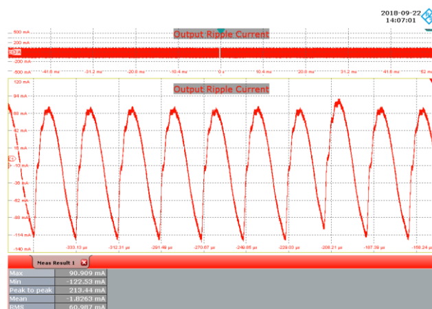
Figure 109 – 100 VAC, 60 Hz, 36 V LED Load. Upper: I_{OUT} , 50 mA / div., 10 ms / div.
