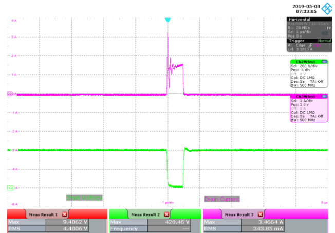
Figure 98 – 277 VAC, Output Shorted. Upper: I_{DRAIN} , 1 A / div. Lower: V_{DRAIN} , 200 V / div., 1 μs / div.
