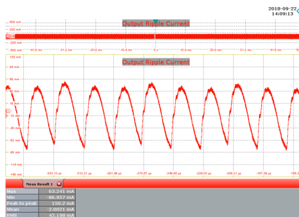
Figure 112 – 277 VAC, 60 Hz, 36 V LED Load. Upper: I_{OUT} , 50 mA / div., 10 ms / div.
