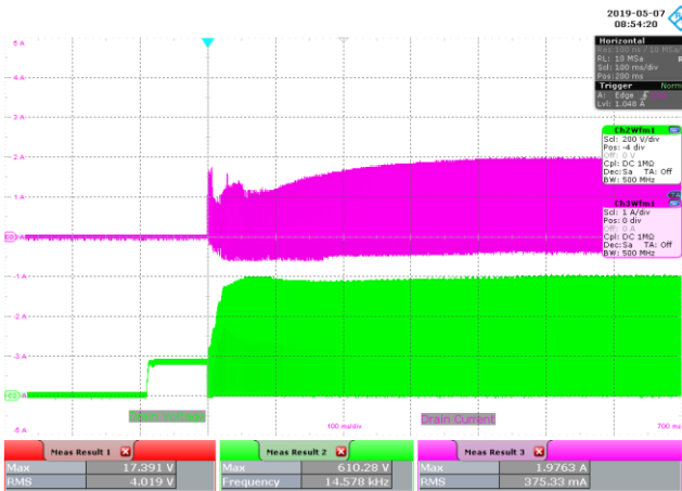
Figure 89 – 100 VAC, 48 V LED Load. Upper: I_{DRAIN} , 1 A / div. Lower: V_{DRAIN} , 200 V / div., 100 ms / div.
