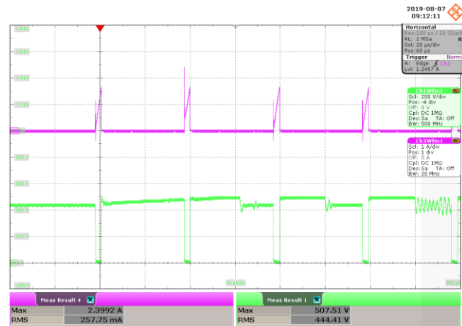
Figure 94 – 305 VAC, 48 V LED Load. Upper: I_{DRAIN} , 1 A / div. Lower: V_{DRAIN} , 200 V / div., 20 μs / div.
