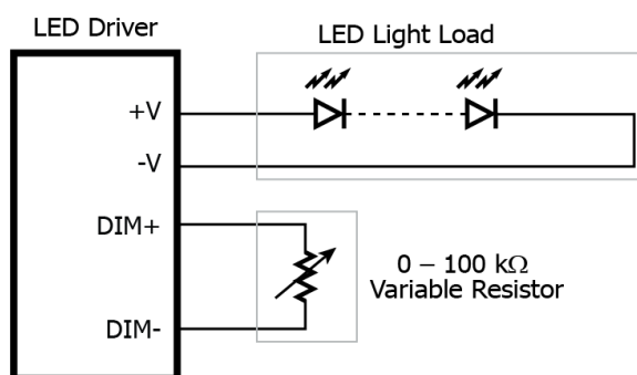
Figure 42 – 0 \Omega - 100 k \Omega Variable Resistor Dimming Set-up.
