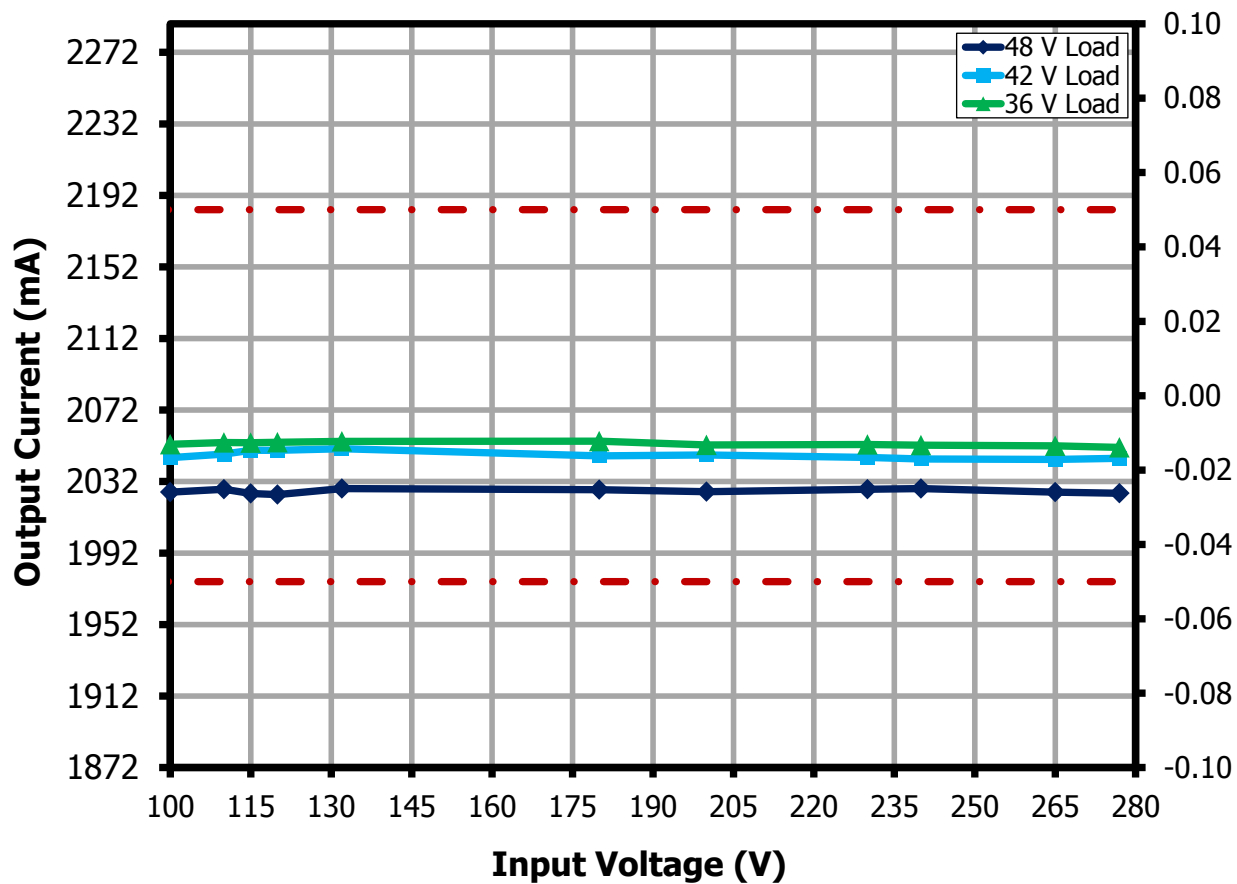
Figure 30 – Current Regulation vs. Line and LED Load.
