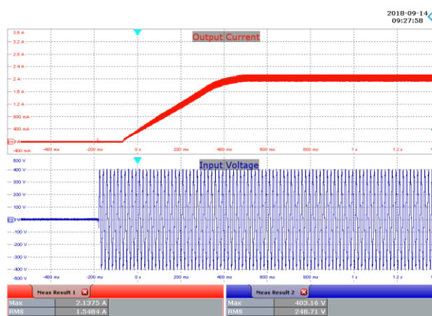
Figure 58 – 277 VAC, 36 V LED, Output Rise. Upper: I_{OUT} , 400 mA / div. Lower: V_{IN} , 100 V / div., 200 ms / div.
