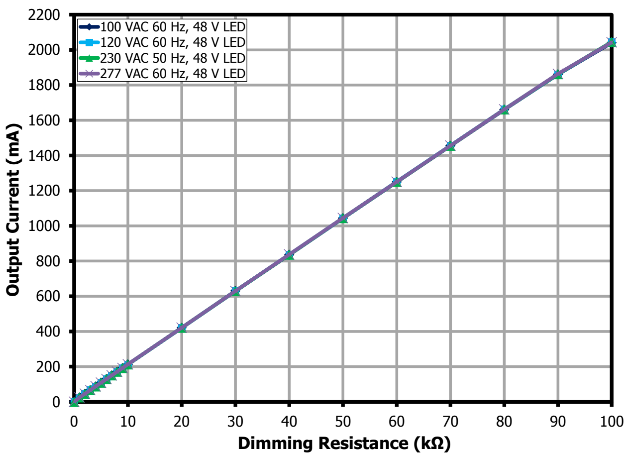
Figure 43 – 0 \Omega - 100 k \Omega Variable Resistor Dimming Curve at 48 V LED Load.
