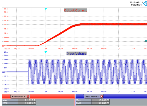
Figure 51 – 100 VAC, 48 V LED, Output Rise. Upper: I_{OUT} , 400 mA / div. Lower: V_{IN} , 50 V / div., 200 ms / div.
