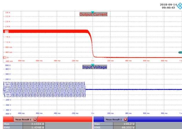
Figure 63 – 100 VAC, 36 V LED, Output Fall. Upper: I_{OUT} , 400 mA / div. Lower: V_{IN} , 100 V / div., 200 ms / div.
