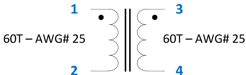
Figure 20 – Common Mode Choke Electrical Diagram.
