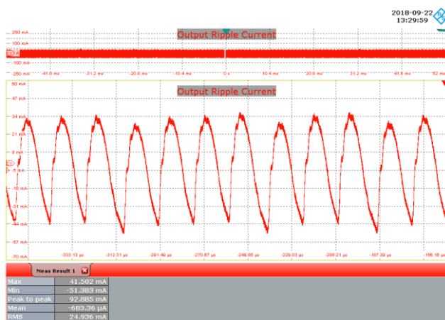
Figure 105 – 100 VAC, 60 Hz, 48 V LED Load. Upper: I_{OUT} , 50 mA / div., 10.4 ms / div.
