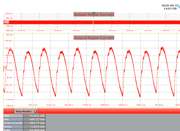
Figure 110 – 120 VAC, 20 Hz, 36 V LED Load. Upper: I_{OUT} , 50 mA / div., 10 ms / div.
