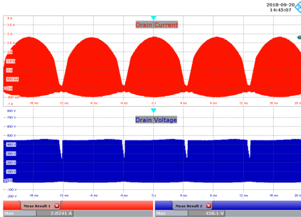
Figure 67 – 100 VAC, 48 V LED Load. Upper: I_{DRAIN} , 500 mA / div. Lower: V_{DRAIN} , 100 V / div., 4 ms / div.
