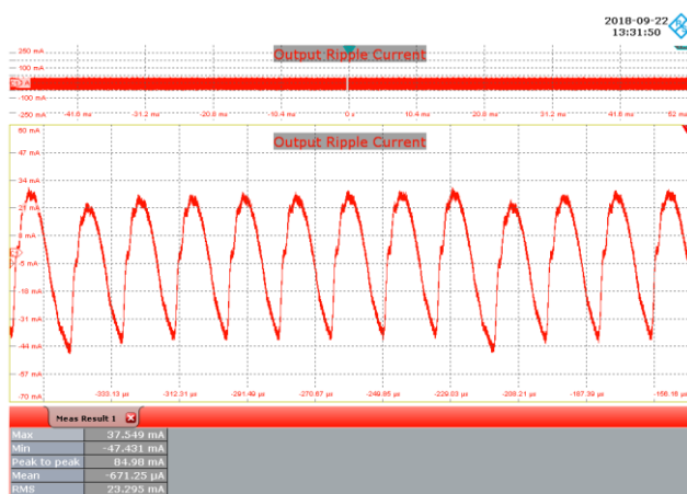
Figure 107 – 230 VAC, 50 Hz, 48 V LED Load. Upper: I_{OUT} , 50 mA / div., 10.4 ms / div.
