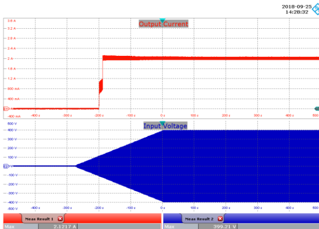
Figure 152 – Brown-in Test at 1 V / s. Ch1: I_{OUT} , 400 mA / div. Ch2: V_{IN} , 100 V / div. Time Scale: 100 s / div.
