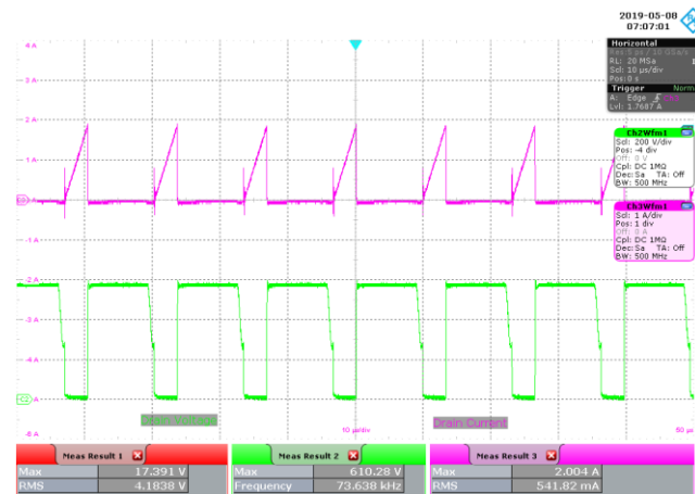
Figure 82 – 120 VAC, 48 V LED Load. Upper: I_{DRAIN} , 1 A / div. Lower: V_{DRAIN} , 200 V / div., 10 μs / div.
