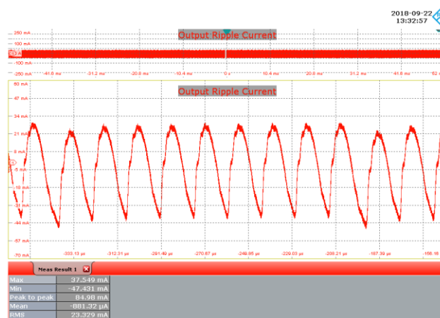
Figure 108 – 277 VAC, 50 Hz, 48 V LED Load. Upper: I_{OUT} , 50 mA / div., 10.4 ms / div.
