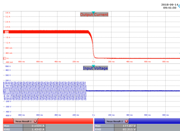
Figure 64 – 120 VAC, 36 V LED, Output Fall. Upper: I_{OUT} , 400 mA / div. Lower: V_{IN} , 100 V / div., 200 ms / div.
