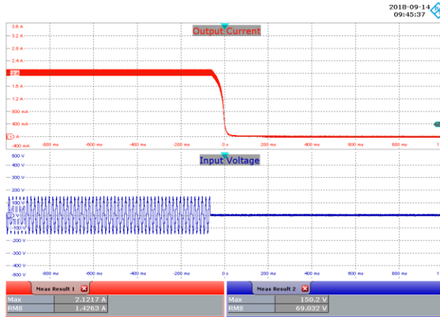
Figure 59 – 100 VAC, 48 V LED, Output Fall. Upper: I_{OUT} , 400 mA / div. Lower: V_{IN} , 100 V / div., 200 ms / div.
