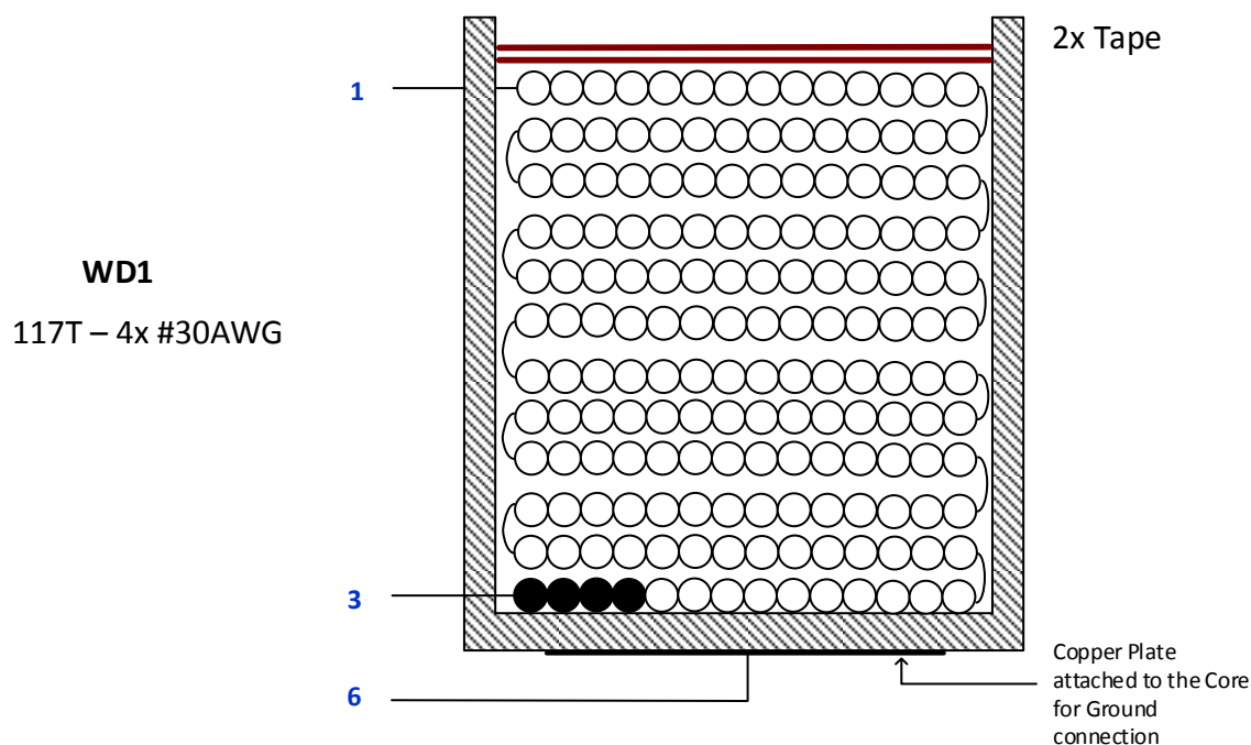
Figure 17 – PFC Inductor Build Diagram.
