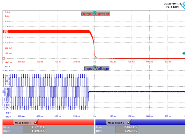
Figure 61 – 230 VAC, 48 V LED, Output Fall. Upper: I_{OUT} , 400 mA / div. Lower: V_{IN} , 100 V / div., 200 ms / div.
