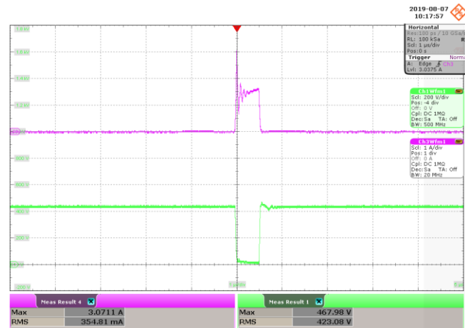
Figure 100 – 305 VAC, Output Shorted. Upper: I_{DRAIN} , 1 A / div. Lower: V_{DRAIN} , 200 V / div., 1 μs / div.
