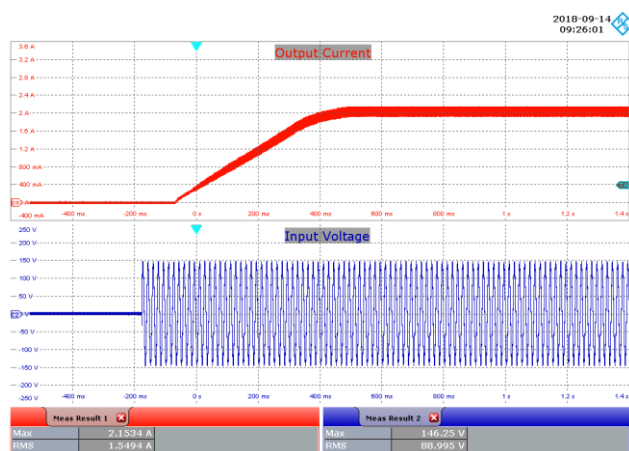
Figure 55 – 100 VAC, 36 V LED, Output Rise. Upper: I_{OUT} , 400 mA / div. Lower: V_{IN} , 50 V / div., 200 ms / div.
