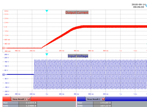
Figure 56 – 120 VAC, 36 V LED, Output Rise. Upper: I_{OUT} , 400 mA / div. Lower: V_{IN} , 50 V / div., 200 ms / div.
