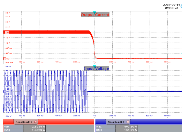
Figure 66 – 277 VAC, 36 V LED, Output Fall. Upper: I_{OUT} , 400 mA / div. Lower: V_{IN} , 100 V / div., 200 ms / div.
