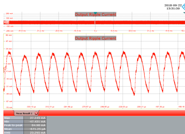
Figure 106 – 120 VAC, 60 Hz, 48 V LED Load. Upper: I_{OUT} , 50 mA / div., 10.4 ms / div.
