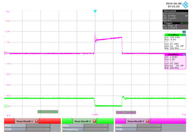
Figure 96 – 100 VAC, Output Shorted. Upper: I_{DRAIN} , 1 A / div. Lower: V_{DRAIN} , 200 V / div., 1 μs / div.
