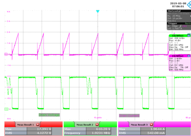
Figure 80 – 100 VAC, 48 V LED Load. Upper: I_{DRAIN} , 1 A / div. Lower: V_{DRAIN} , 200 V / div., 10 μs / div.
