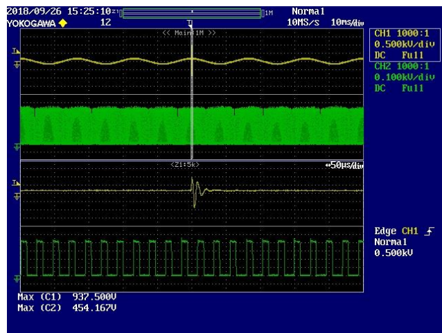
Figure 138 – (+) 2.5 kV Ring Wave Surge, 90° Phase Angle. Lower: V_{DRAIN} , 100 V / div., 10 ms / div. Peak V_{DRAIN} : 454.17 V.
