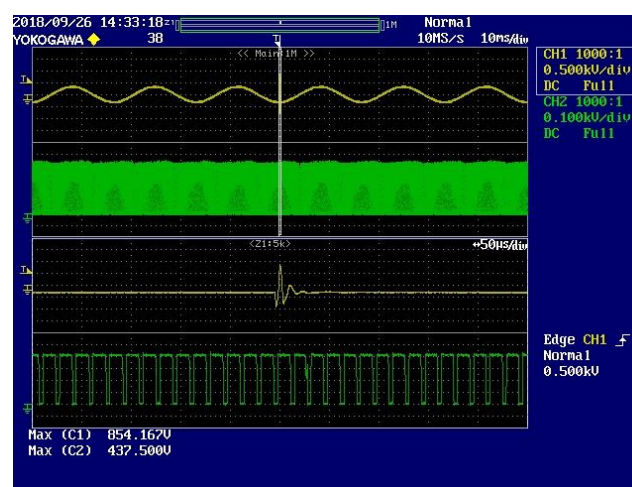
Figure 149 – (-) 2.5 kV Ring Wave Surge, 270° Phase Angle. Lower: V_{DRAIN} , 100 V / div., 10 ms / div. Peak V_{DRAIN} : 437.50 V.
