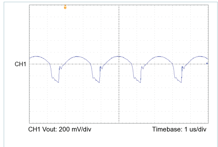
Figure 18 — Output voltage ripple, V_{IN} = 28\text{V} , V_{OUT} = 3.3\text{V} , C_{OUT\_EXT} = 1000\mu\text{F} , R_{LOAD} = 0.091\Omega
