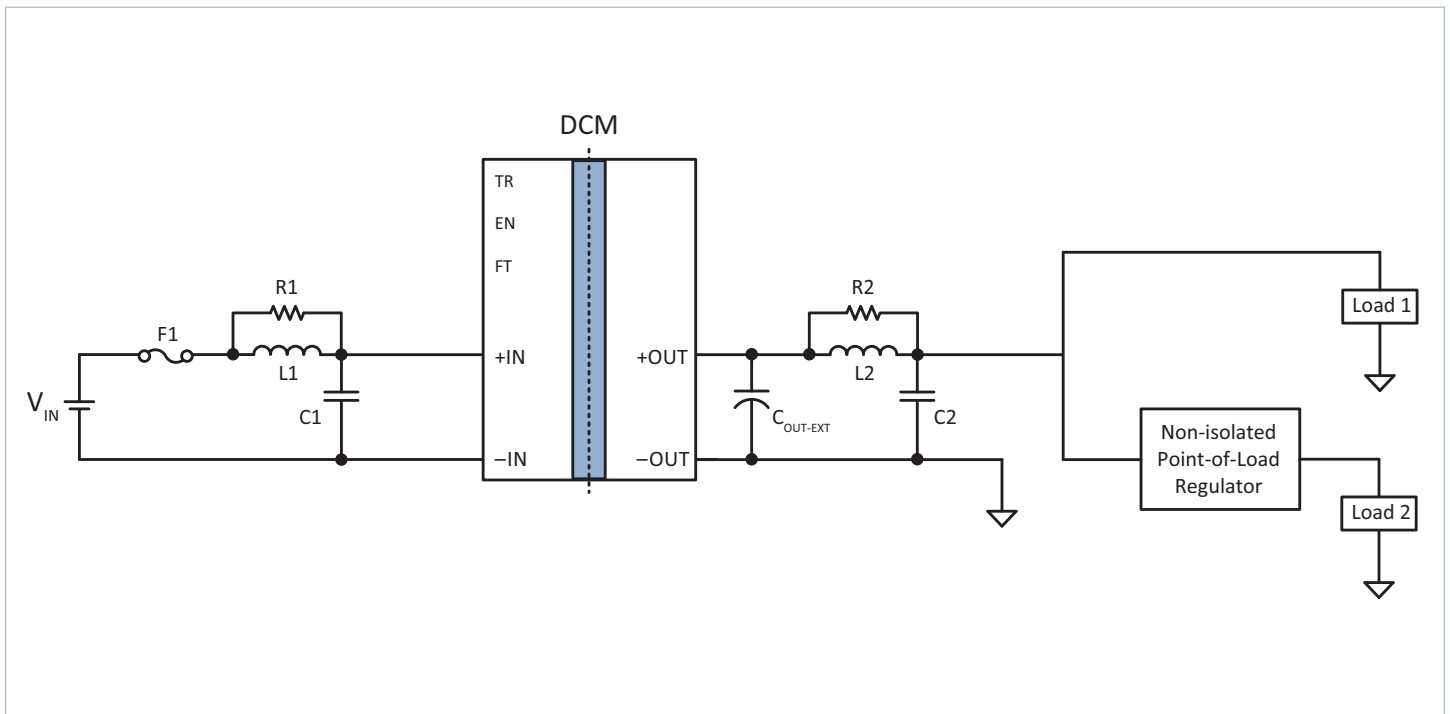
Typical Application 1: Single DCM4623xD2K04A5y7z, to a non-isolated regulator, and direct to load
