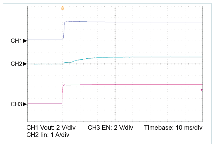
Figure 14 — Startup from EN, V_{IN} = 270\text{ V} , C_{OUT\_EXT} = 10000\text{ }\mu\text{F} , R_{LOAD} = 0.073\text{ }\Omega
