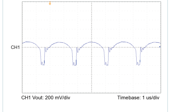
Figure 16 — Output voltage ripple, V_{IN} = 270\text{ V} , V_{OUT} = 3.3\text{ V} , C_{OUT\_EXT} = 1000\text{ }\mu\text{F} , R_{LOAD} = 0.073\text{ }\Omega
