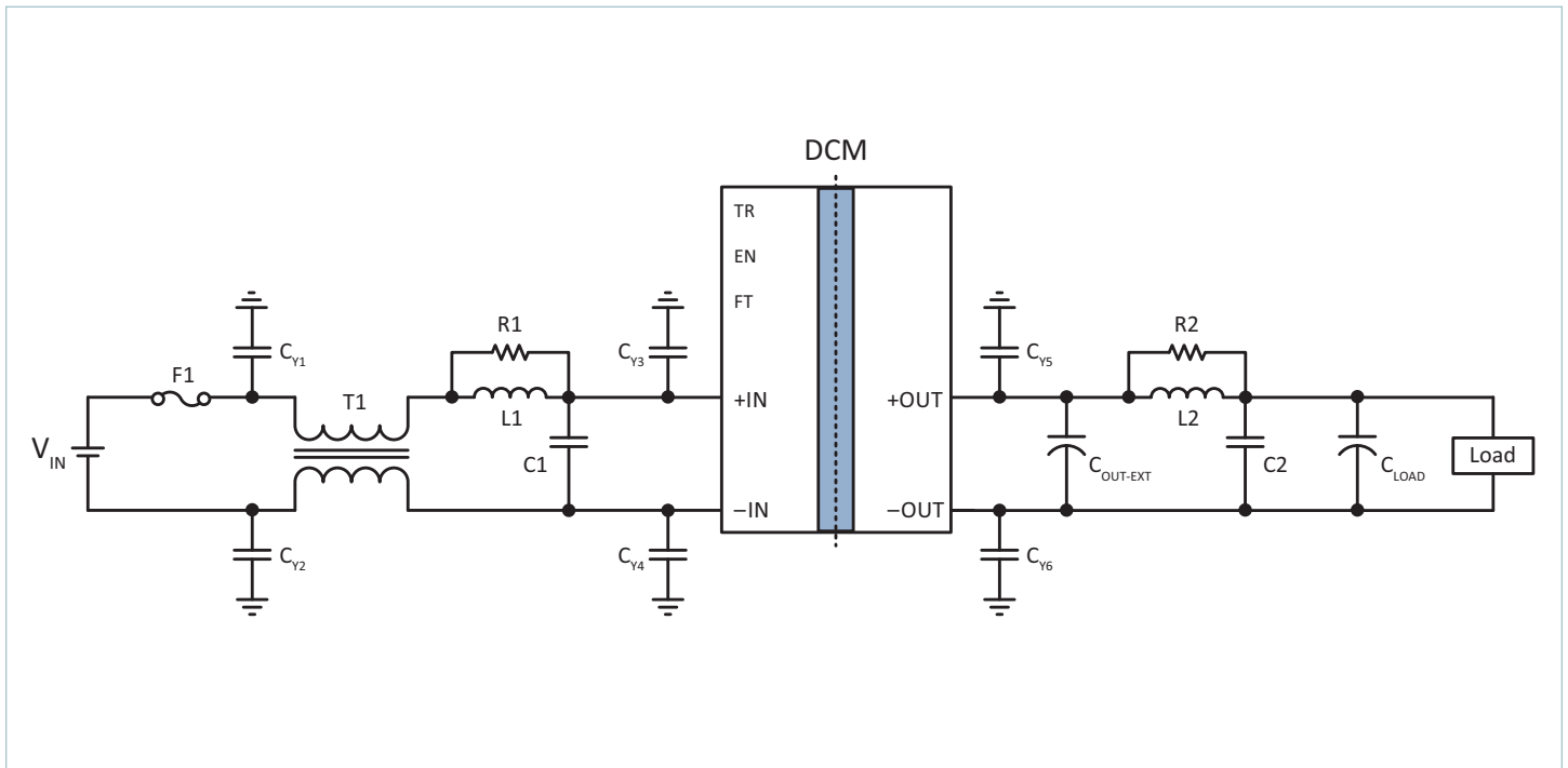
Typical Application 2: Single DCM4623xD2K04A5y7z with common- and differential-mode input filters
