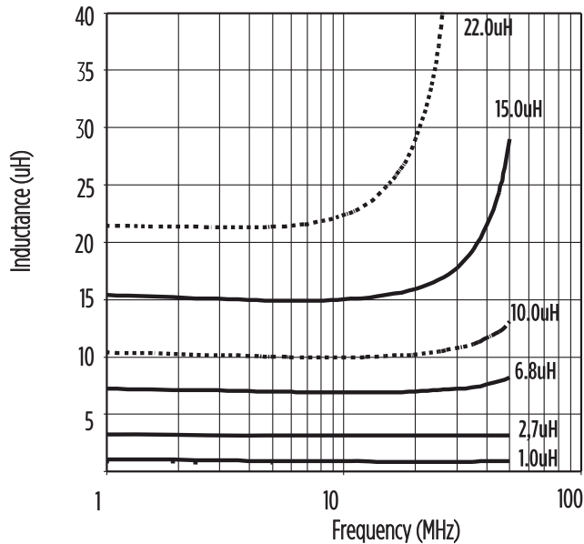
Typical Inductance vs Frequency
