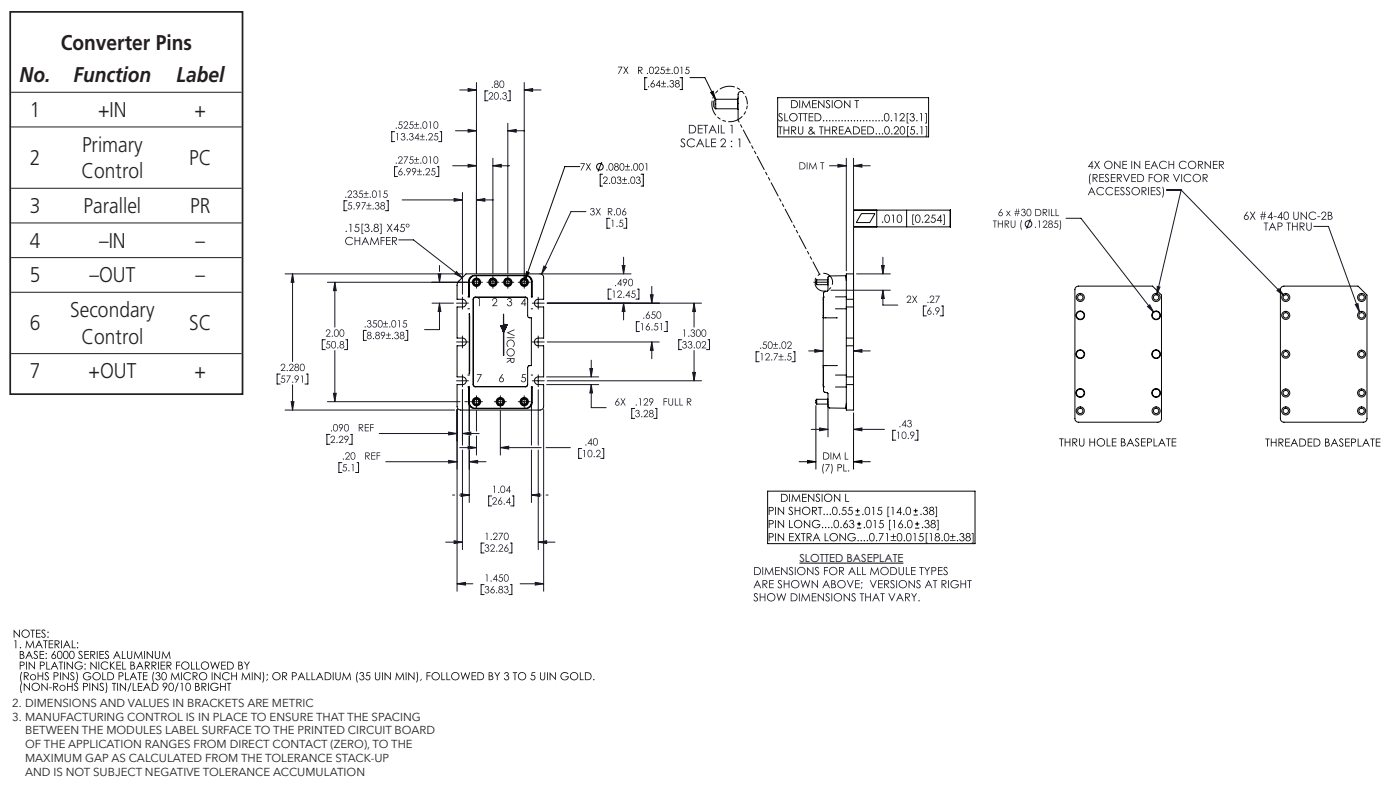
Figure 13 — Module outline
