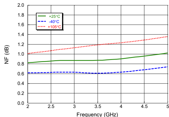
LNA IN to RX OUT Noise Figure 11 - RX Mode
