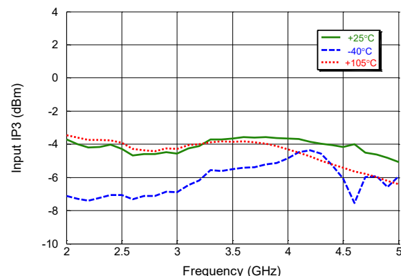
LNA IN to RX OUT Input IP3 - RX Mode
