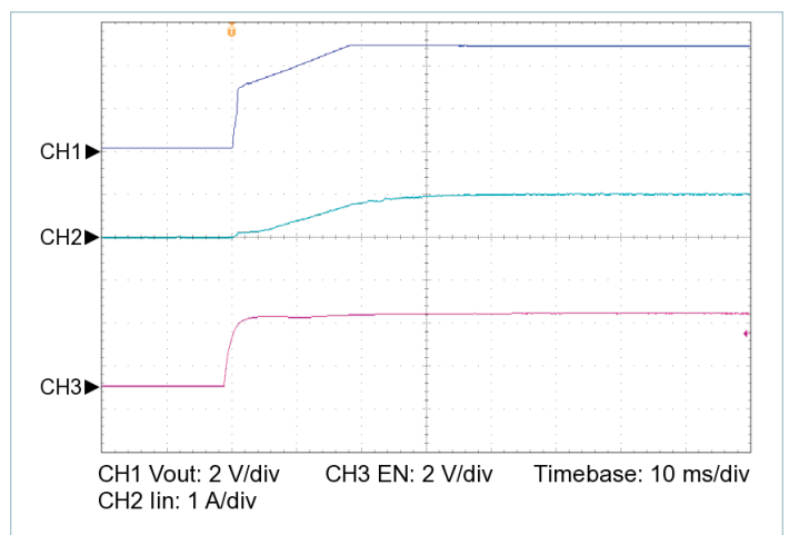
Figure 14 — Startup from EN, V_{IN} = 270\text{ V} , C_{OUT\_EXT} = 10000\text{ }\mu\text{F} , R_{LOAD} = 0.100\text{ }\Omega
