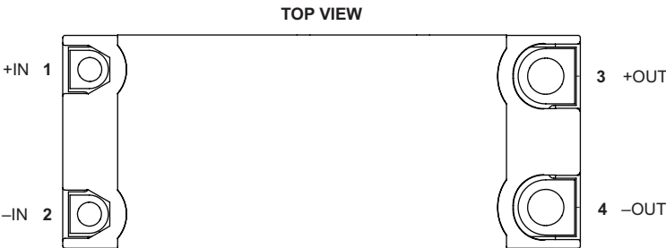
PFM4914 VIA - Chassis Mount - Terminals Up
