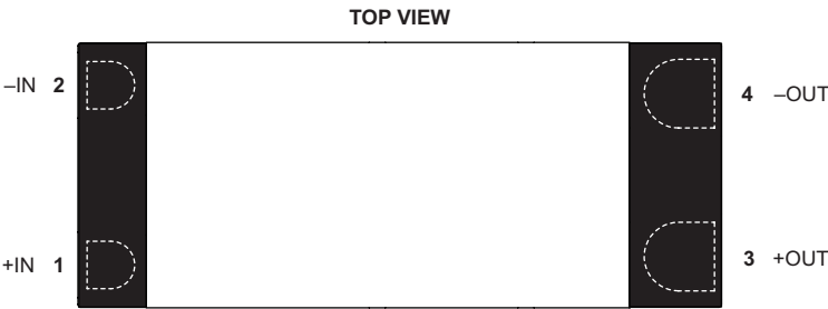
PFM4914 VIA - PCB Mount - Pins Down
