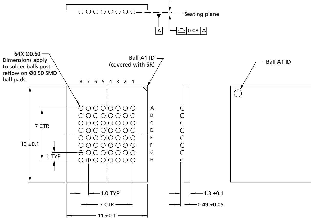
Figure 26: 64-Ball LBG A – 11mm x 13mm (Package Code: PC)
