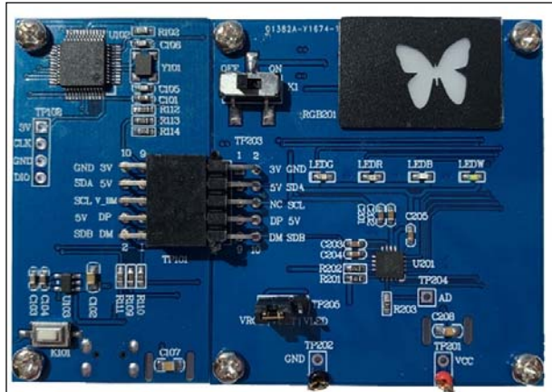
Figure 1: Photo of IS31FL3197-QFLS2 Evaluation Board
