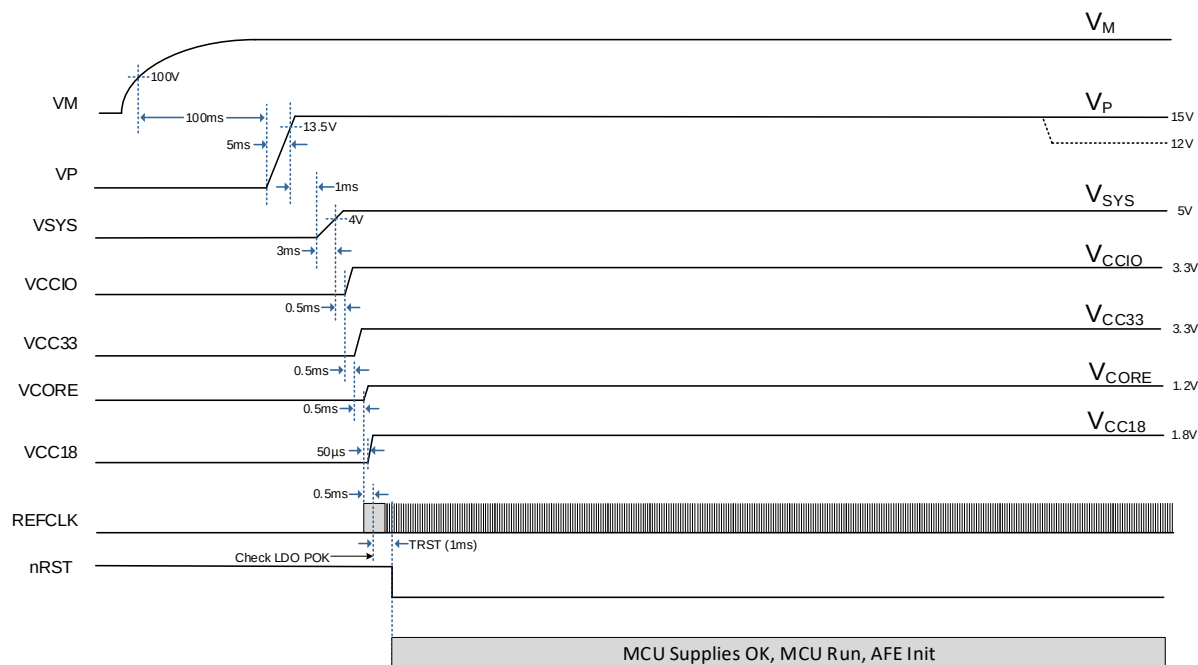
Figure 10-5 Power-Up Sequence
