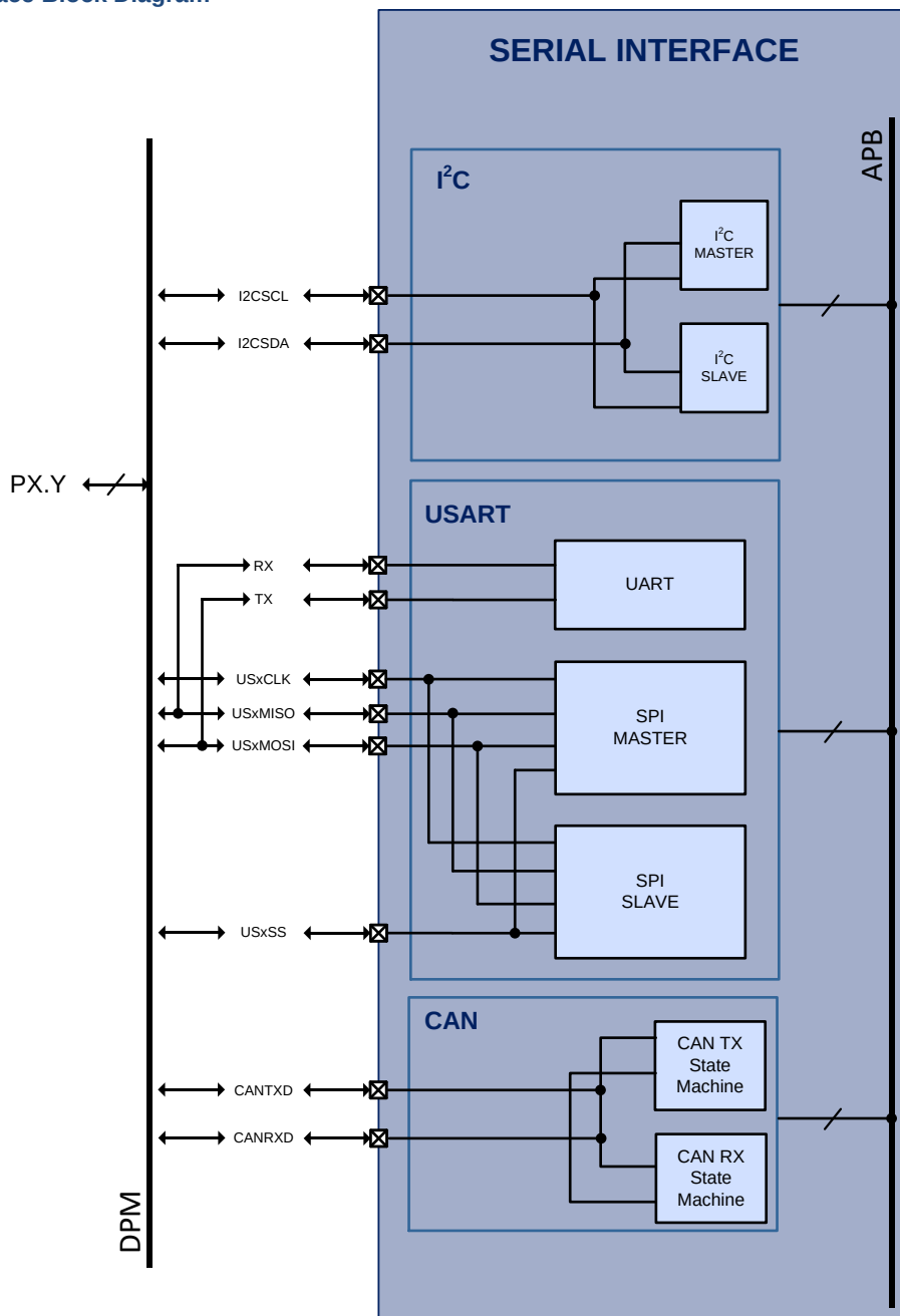
Figure 19-1 Serial Interface Block Diagram
