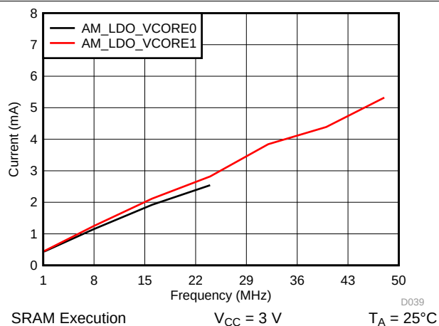
Figure 5-10. Frequency vs Current Consumption
