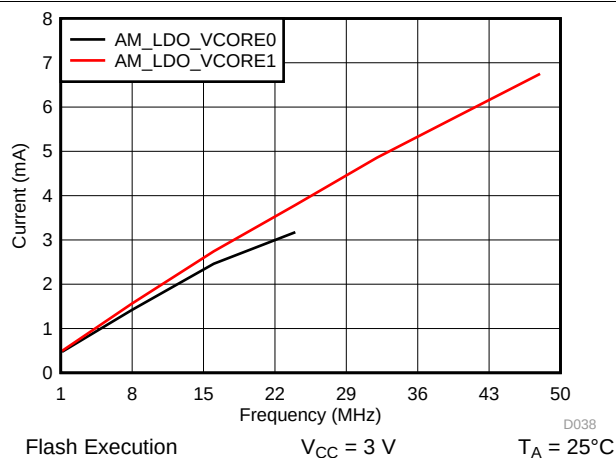
Figure 5-9. Frequency vs Current Consumption
