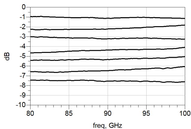
Relative Attenuation
