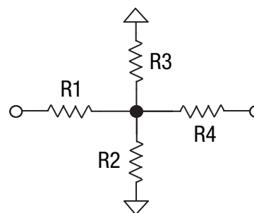
Figure 9. Circuit Topology (1 to 5 dB Attenuators)
