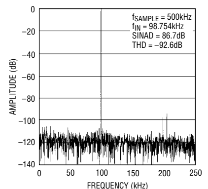
LTC1608 4096 Point FFT
