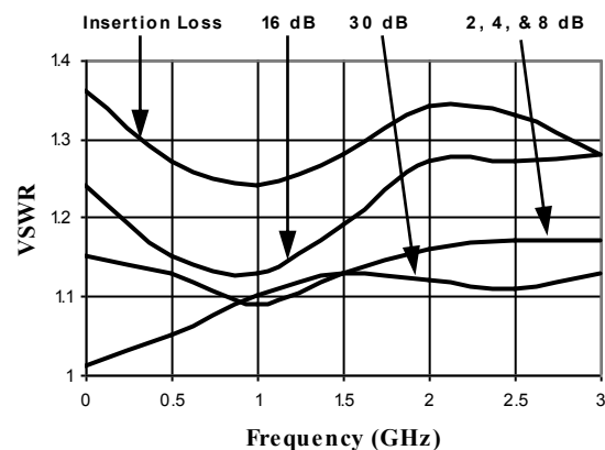
Typical RF2 VSWR
