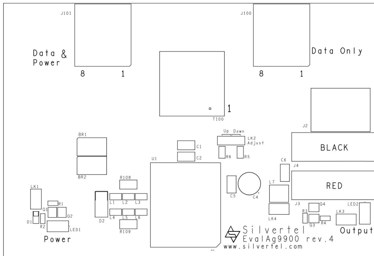
Figure 1: EvalAg9900 Board Layout
