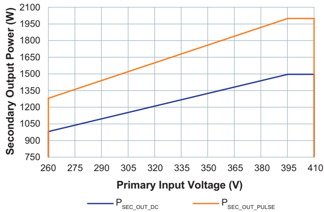
Figure 2 — Specified electrical operating area using rated R_{SEC\_HOT}
