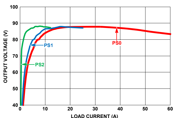
FIGURE 2. V_{OUT} vs LOAD
