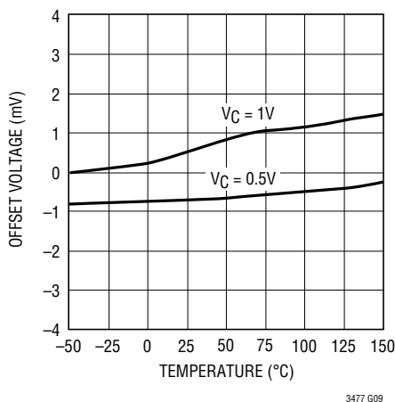
Feedback Amplifier Offset Voltage
