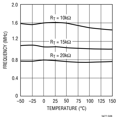
Oscillator Frequency
