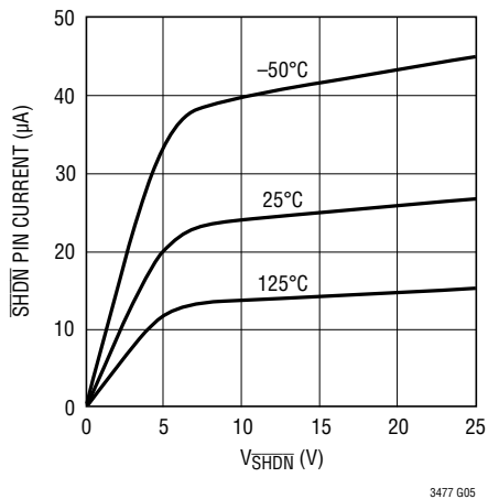
\overline{SHDN} Pin Current
