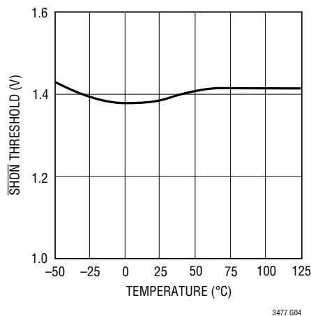
\overline{SHDN} Pin Turn-On Threshold
