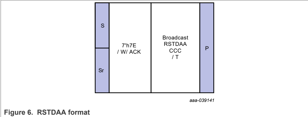
Figure 6. RSTDAA format
