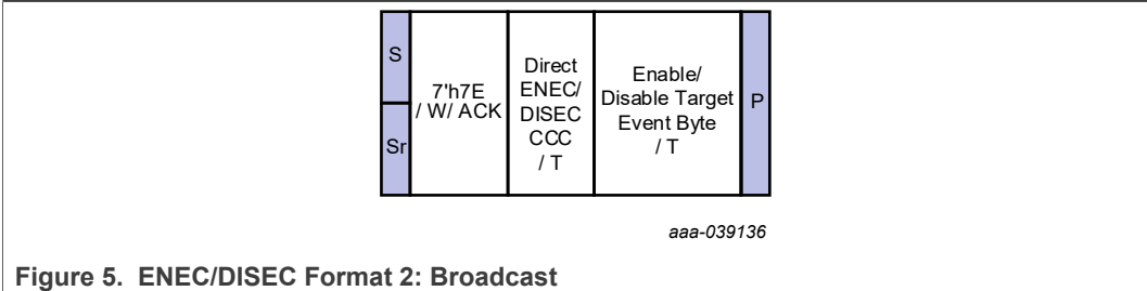
Figure 5. ENEC/DISEC Format 2: Broadcast
