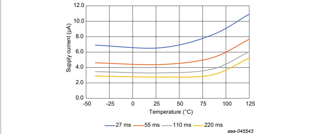
Figure 25. Supply current versus conversion time and temperature (V CC = 1.8 V, bus inactive)
