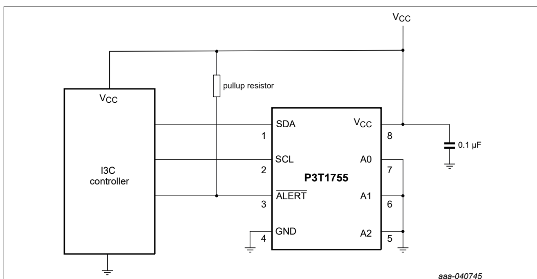
Figure 21. I3C typical application
